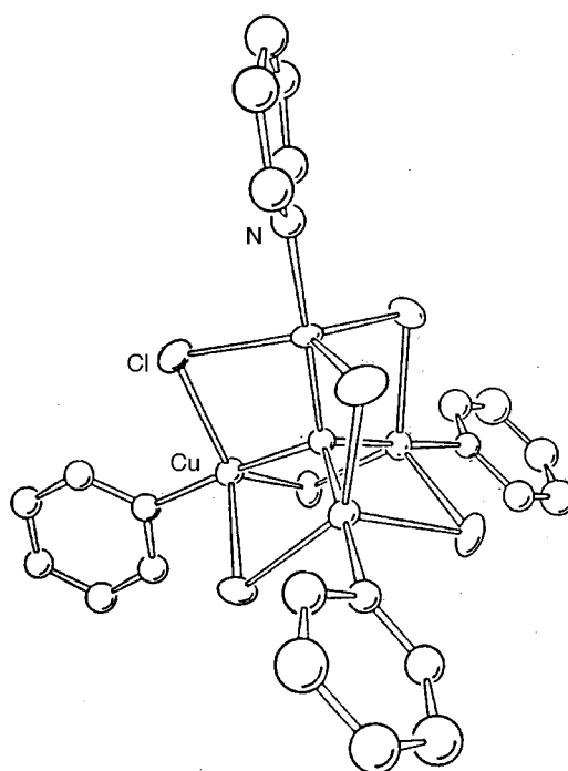
Fig. 1 Structure of [\text{Cu}_4\text{OCl}_6(\text{py})_4] ( \text{py} = \text{pyridine} ) taken from ref. 2(b)
