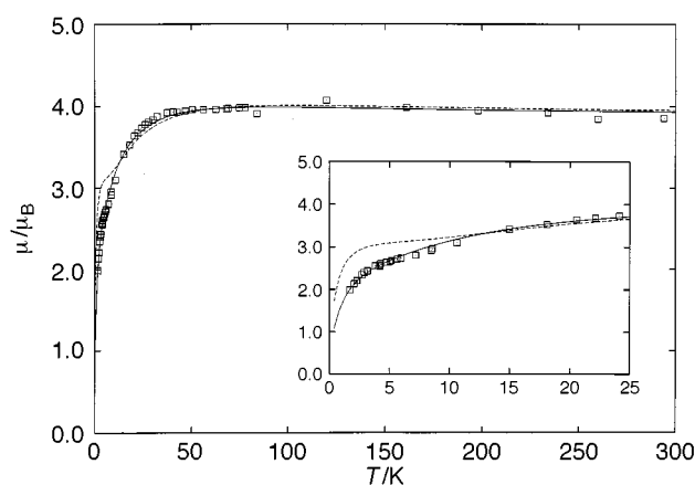
Fig. 4 Magnetic moment \mu_{\text{eff}}/\mu_B of [\text{Cu}_4\text{OCl}_6(\text{py})_4] . \square , Data from ref. 6. Curves calculated as described in the text with d_1 and d_2 (fixed) 3.7 \text{cm}^{-1} : ---, best fit without molecular-field correction; —, best fit including molecular-field correction. Inset: detail of the 0–25 K region
